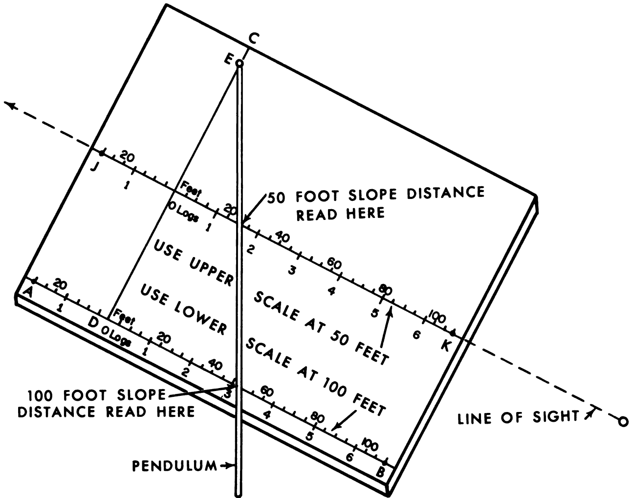
Figure 2-4. Modified Faustman hypsometer.
